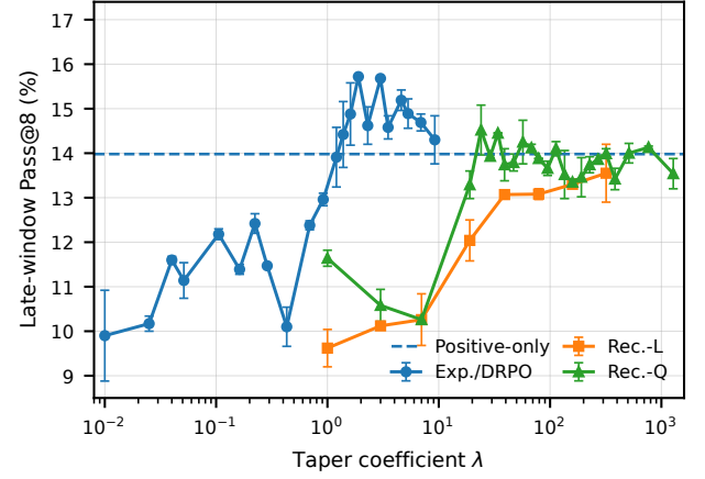
Figure 5: Countdown-0.5B taper-coefficient response. Late-window Pass@8 is shown against the taper coefficient \lambda under the fixed 1,200-step budget. Curves report two-seed late-window means; error bars span the paired seed values, and the dashed horizontal line denotes Positive-only. Exp./DRPO is shown over \lambda \in [0.01, 9.2103] , Reciprocal-Linear through 319, and Reciprocal-Quadratic through 1279.
