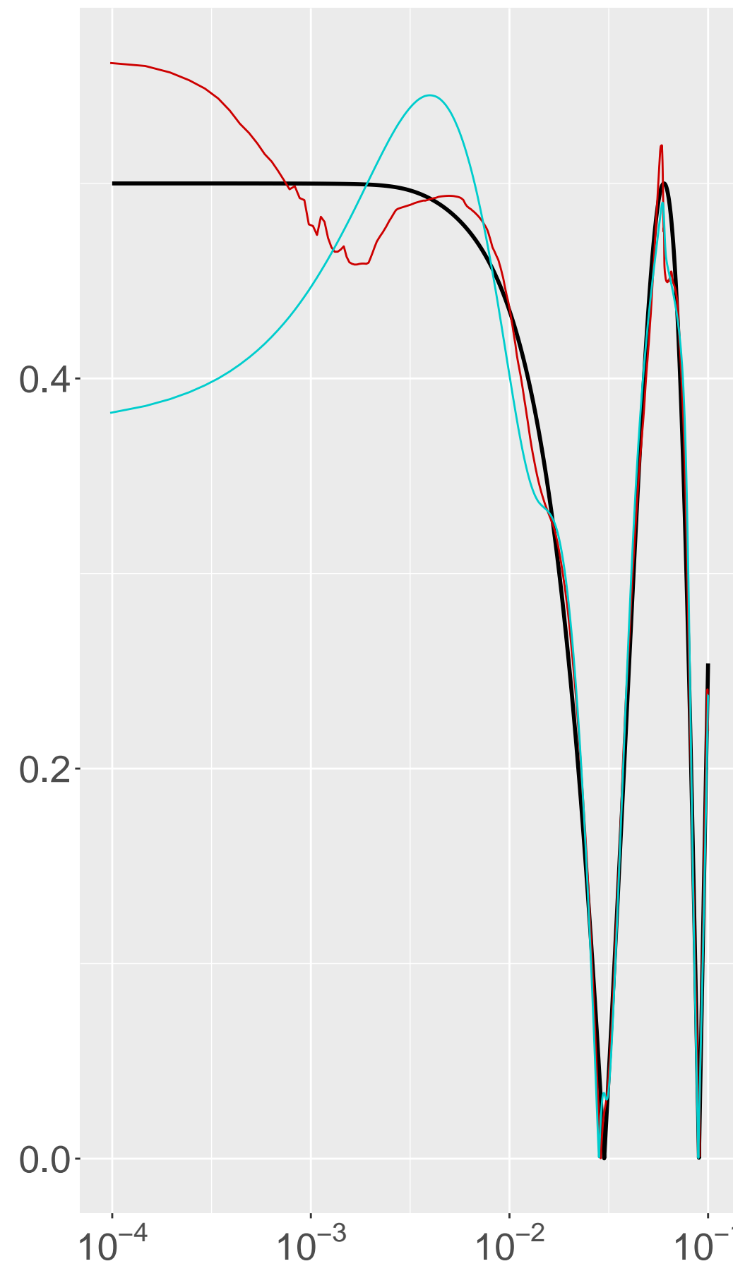
Coherence XZ
