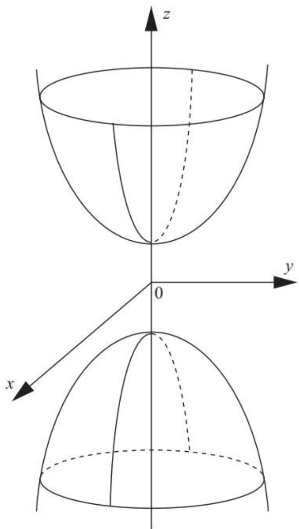
(a) Figure 2-8. 非连通曲面: -y^2 - x^2 + z^2 = 1
