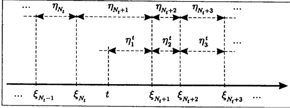
FIGURE 4. The random variables \eta_1^t, \eta_2^t, \eta_3^t, \dots
