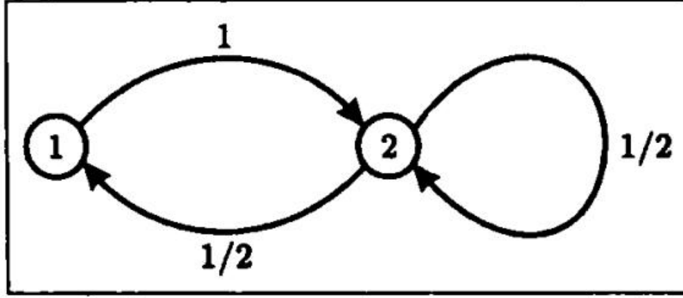
FIGURE 1. Transition probabilities of the Markov chain in Exercise 2.25
