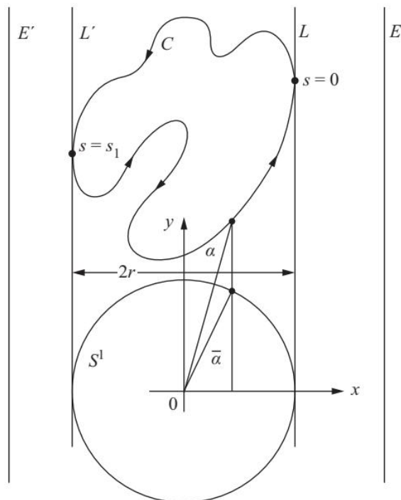
(b) Figure 1-24. 等周不等式证明图示
