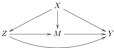
FIGURE 27.1: Causal diagram for mediation analysis
