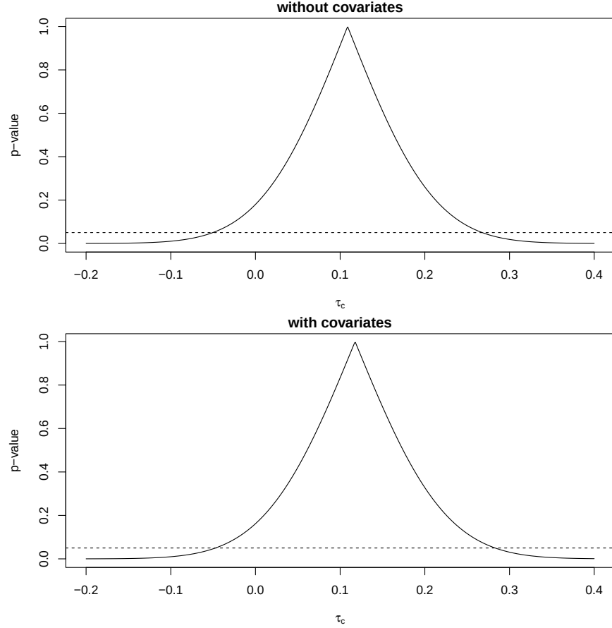
FIGURE 21.1: Confidence interval of \tau_c by inverting tests: upper panel without covariate adjustment, and lower panel with covariate adjustment
