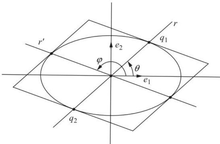
(a) Figure 3-13. The Dupin indicatrix —椭圆点（左）与双曲点（右）的刻画
