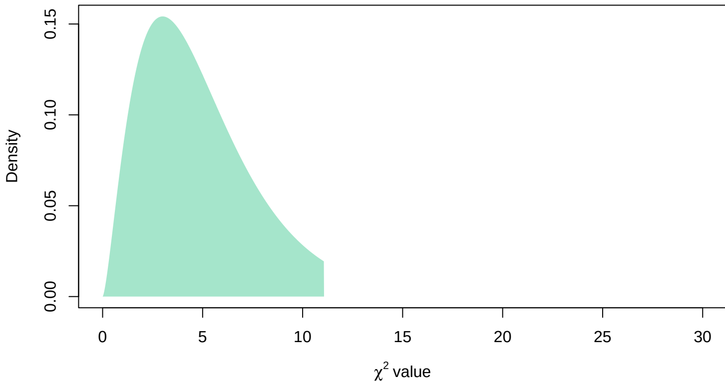
Chi-square Distribution \chi^2(5) for Goodness-of-Fit Test
