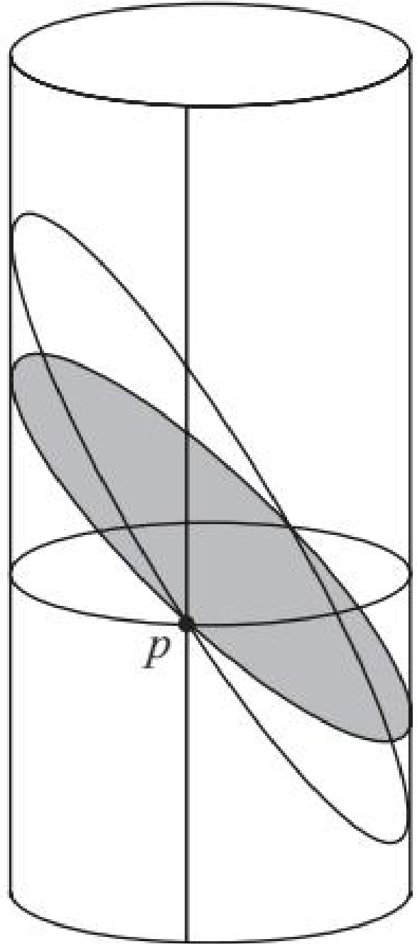
(b) Figure 3-12. Normal sections on a cylinder
