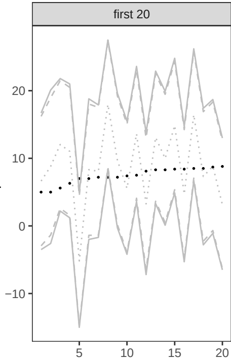
outcomes and predicted values
