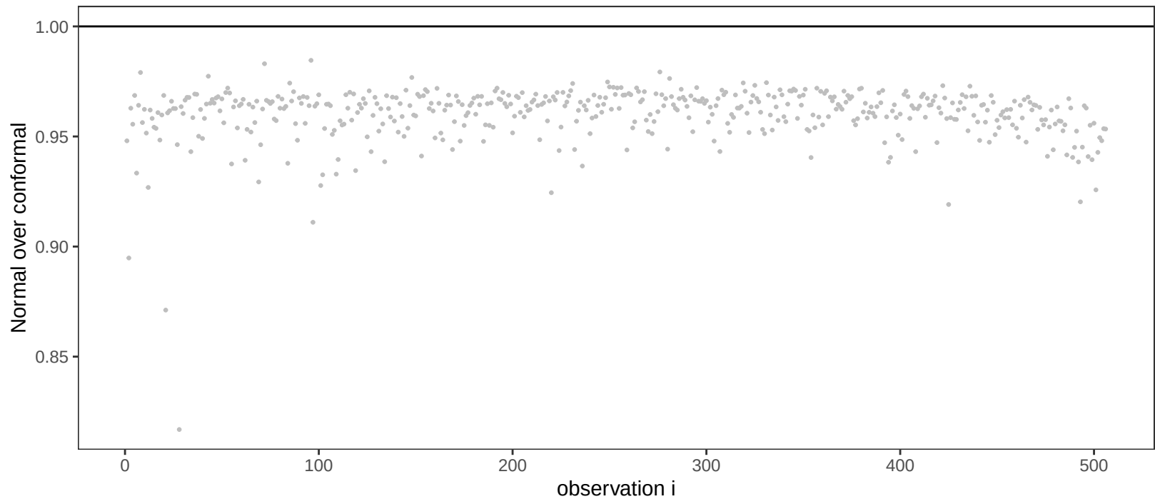
ratio of the lengths of leave-one-out prediction intervals
