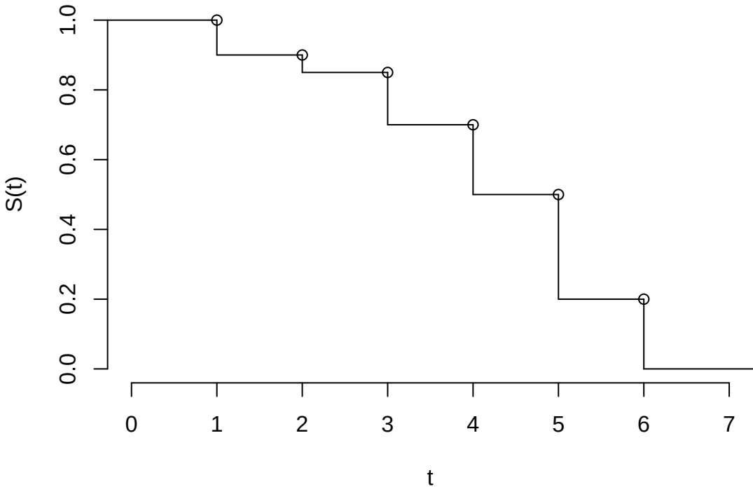
discrete distribution
