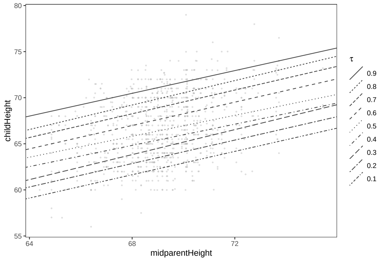
quantile regressions
