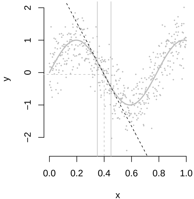
local linear approximation
