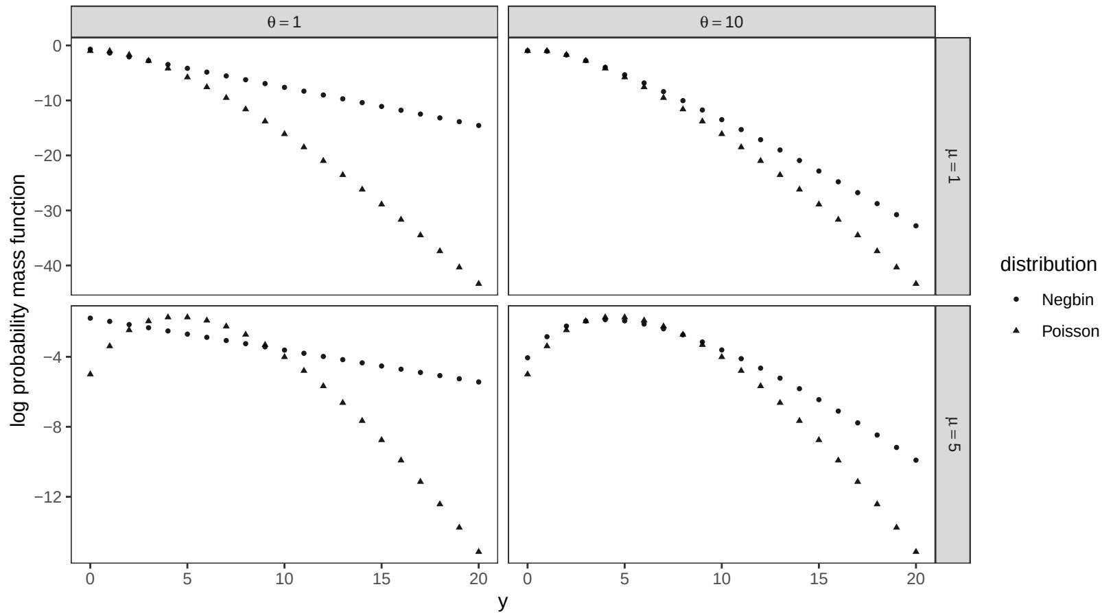
comparing Poisson and Negative Binomial
