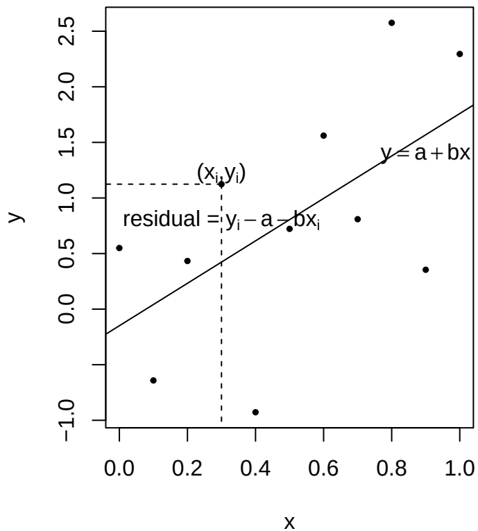
regression
