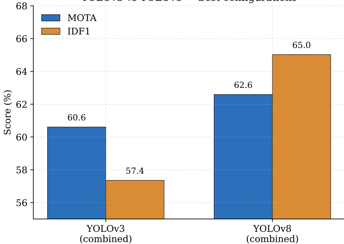
YOLOv3 vs YOLOv8 — best configurations
