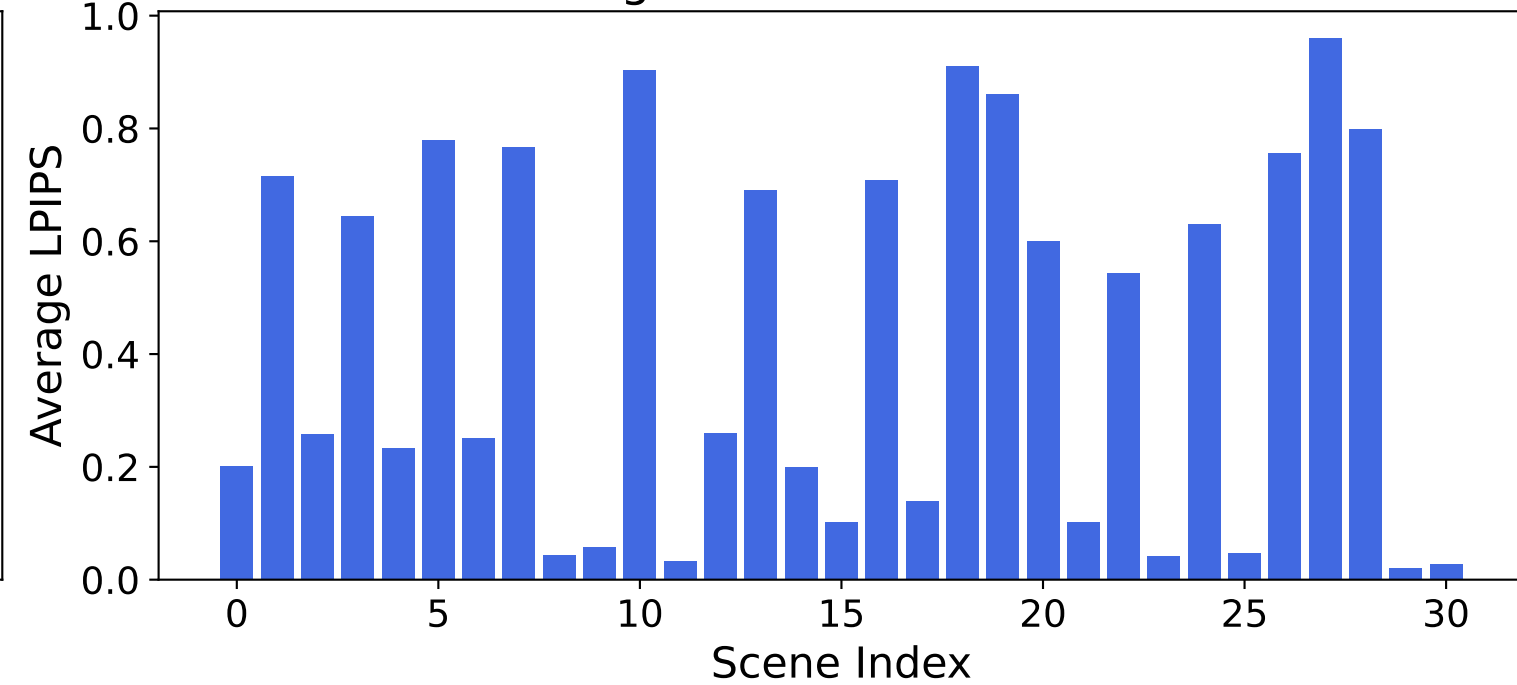
Average LPIPS for Each Scene
