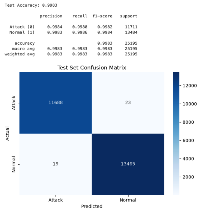
Figure 1: Model Accuracy, Classification Report and Confusion Matrix
