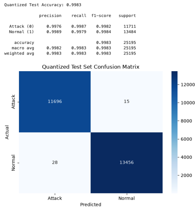
Figure 2: Quantized INT8 Model Accuracy, Classification Report and Confusion Matrix
