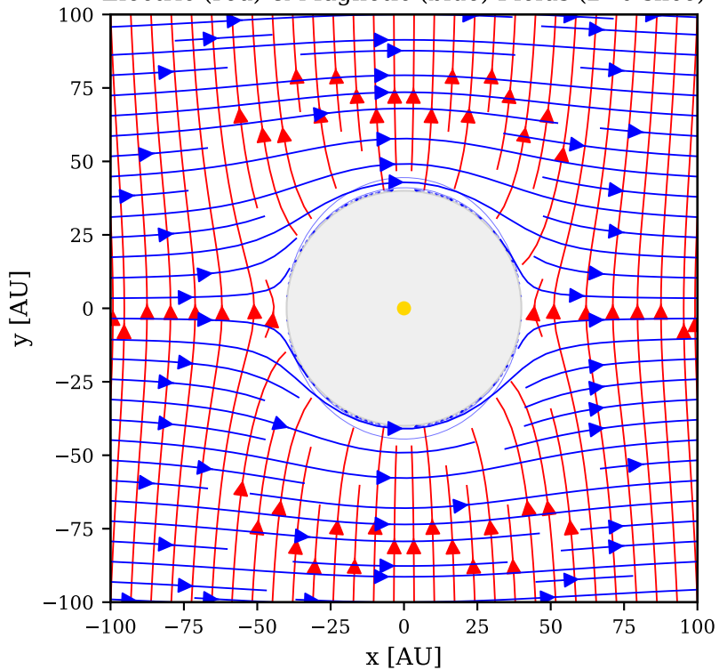
Electric (red) & Magnetic (blue) Fields ( z=0 slice)
