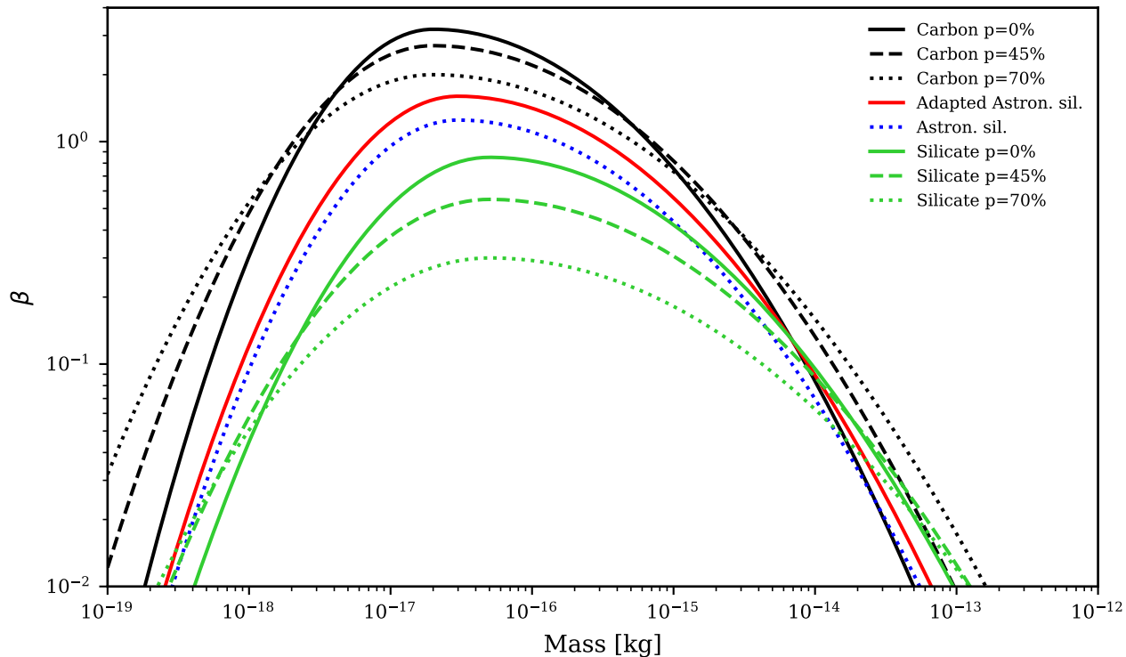
\beta curves for multiple materials
