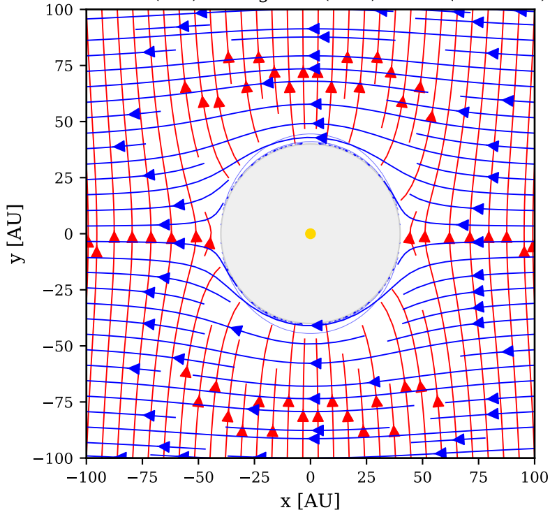
Electric (red) & Magnetic (blue) Fields ( z=0 slice)
