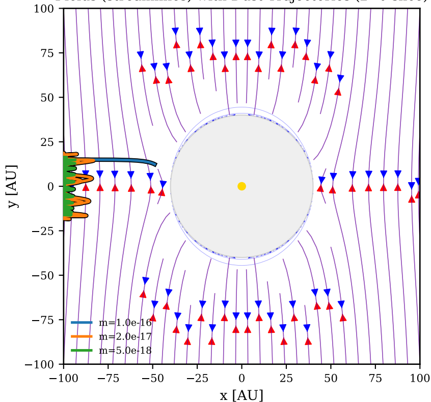
Fields (streamlines) with Dust Trajectories (z=0 slice)
