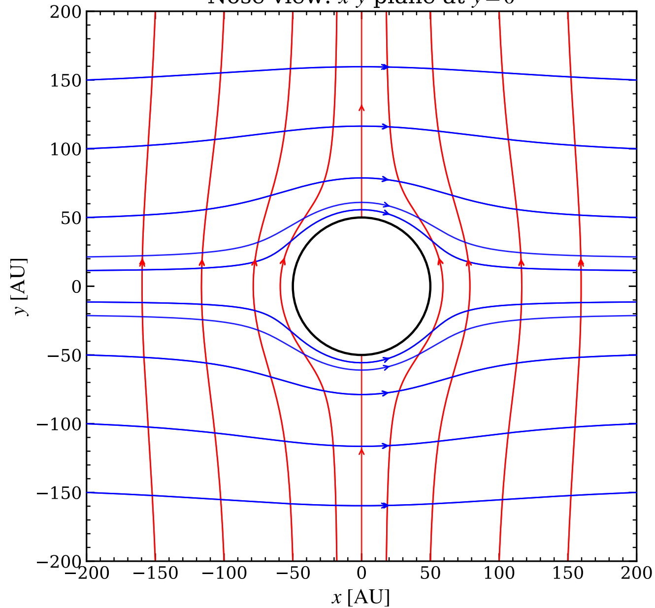
Nose view: x - y plane at y=0
