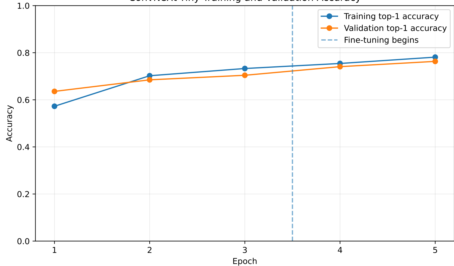
ConvNeXt-Tiny Training and Validation Accuracy
