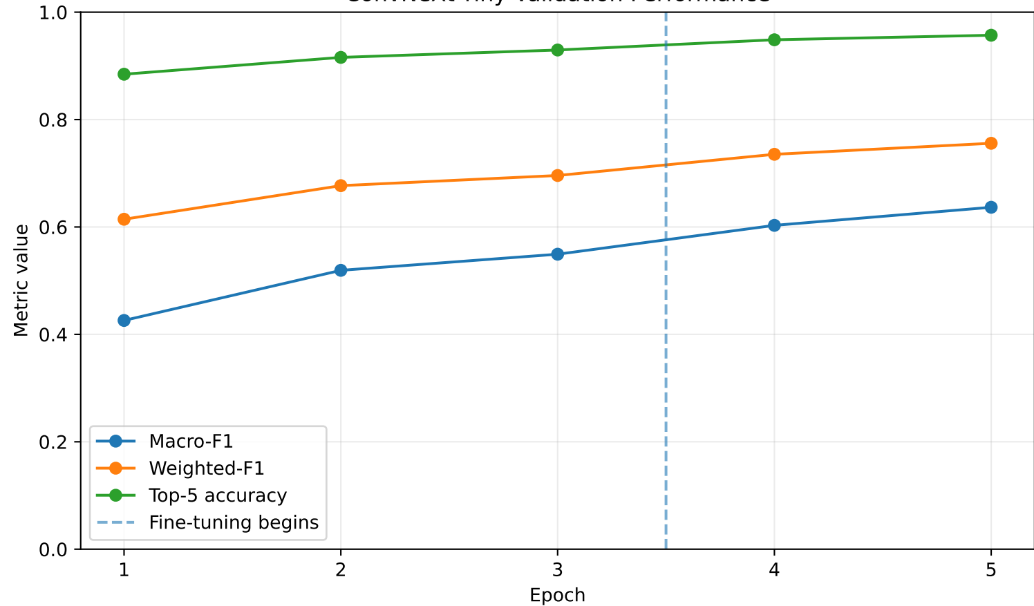
ConvNeXt-Tiny Validation Performance
