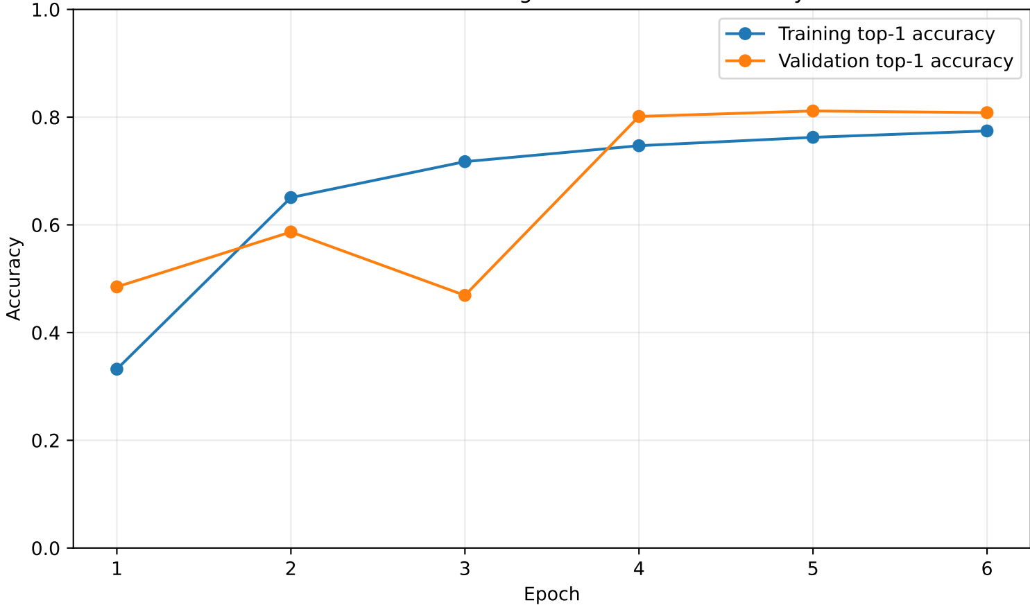
Custom CNN Training and Validation Accuracy
