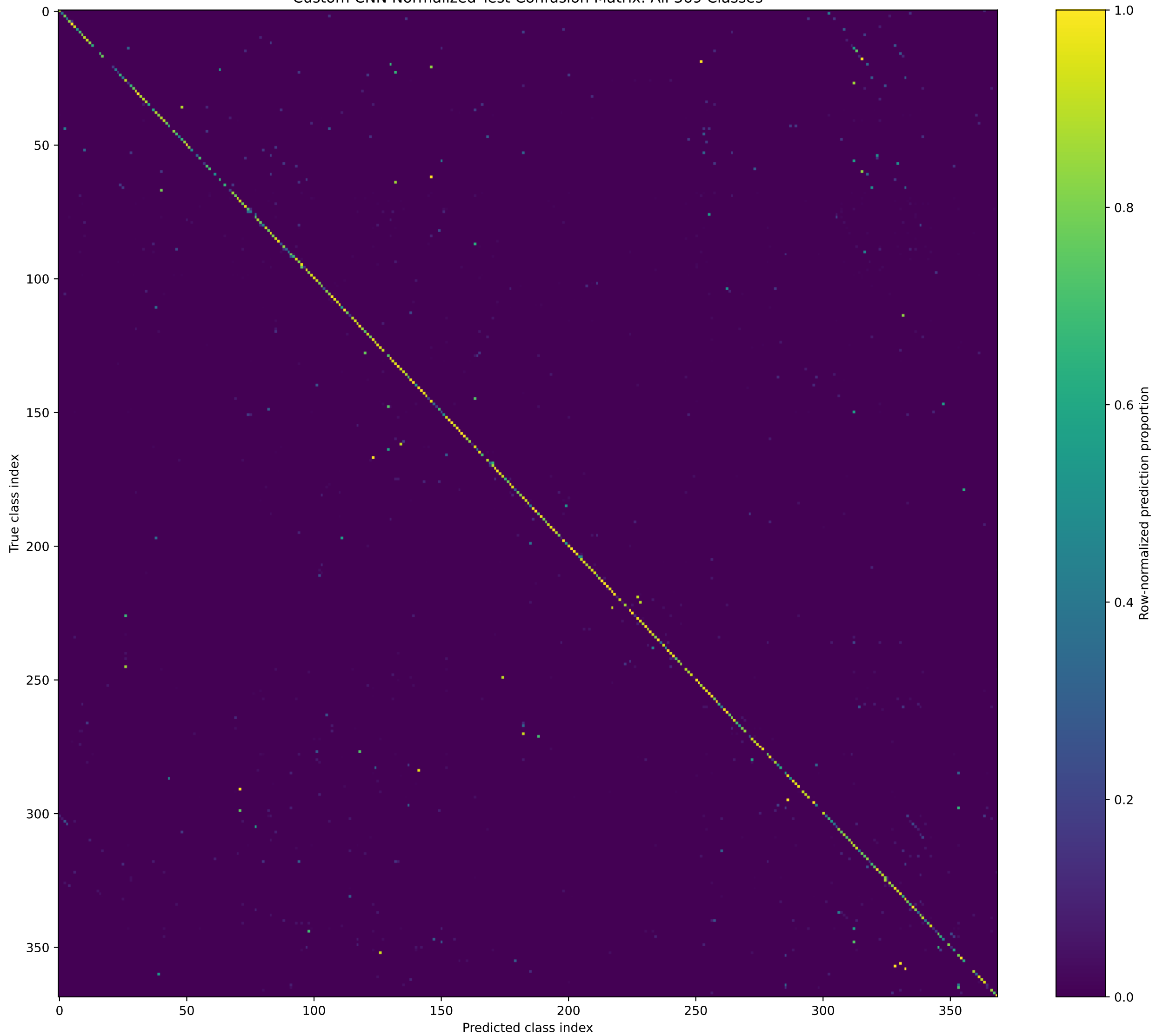
Custom CNN Normalized Test Confusion Matrix: All 369 Classes
