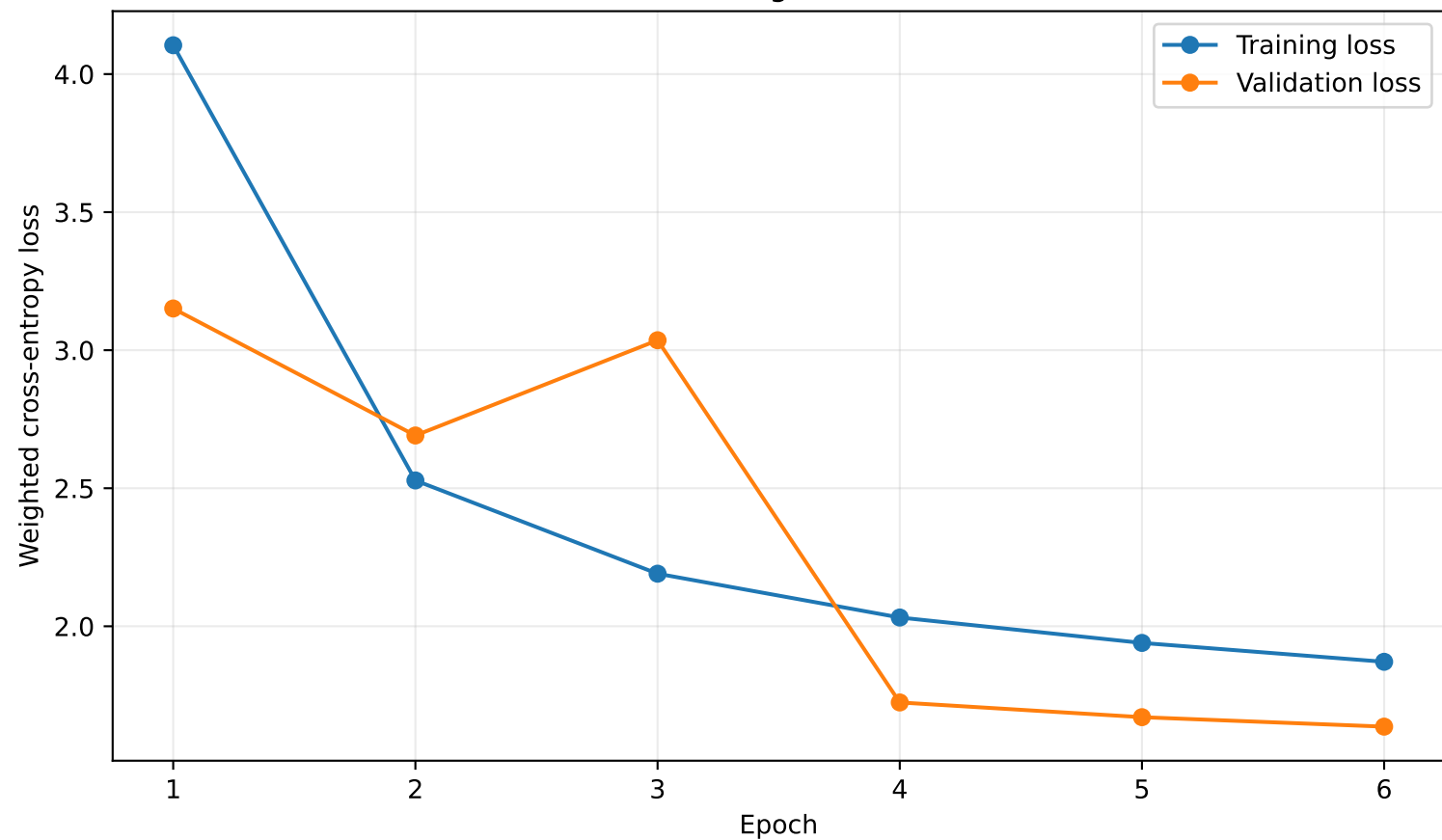
Custom CNN Training and Validation Loss
