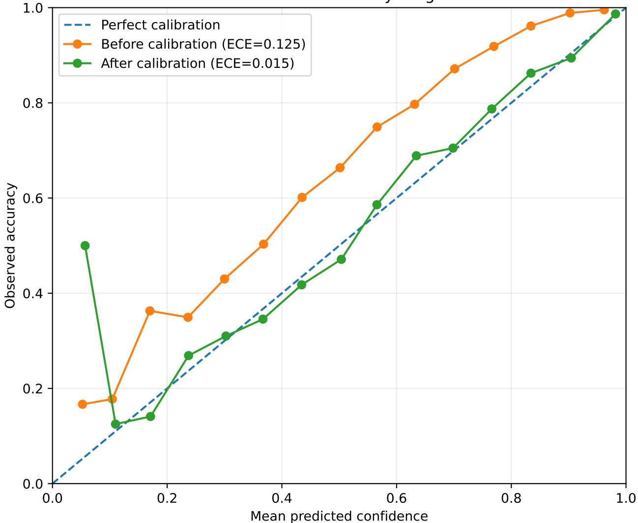
Custom CNN Reliability Diagram
