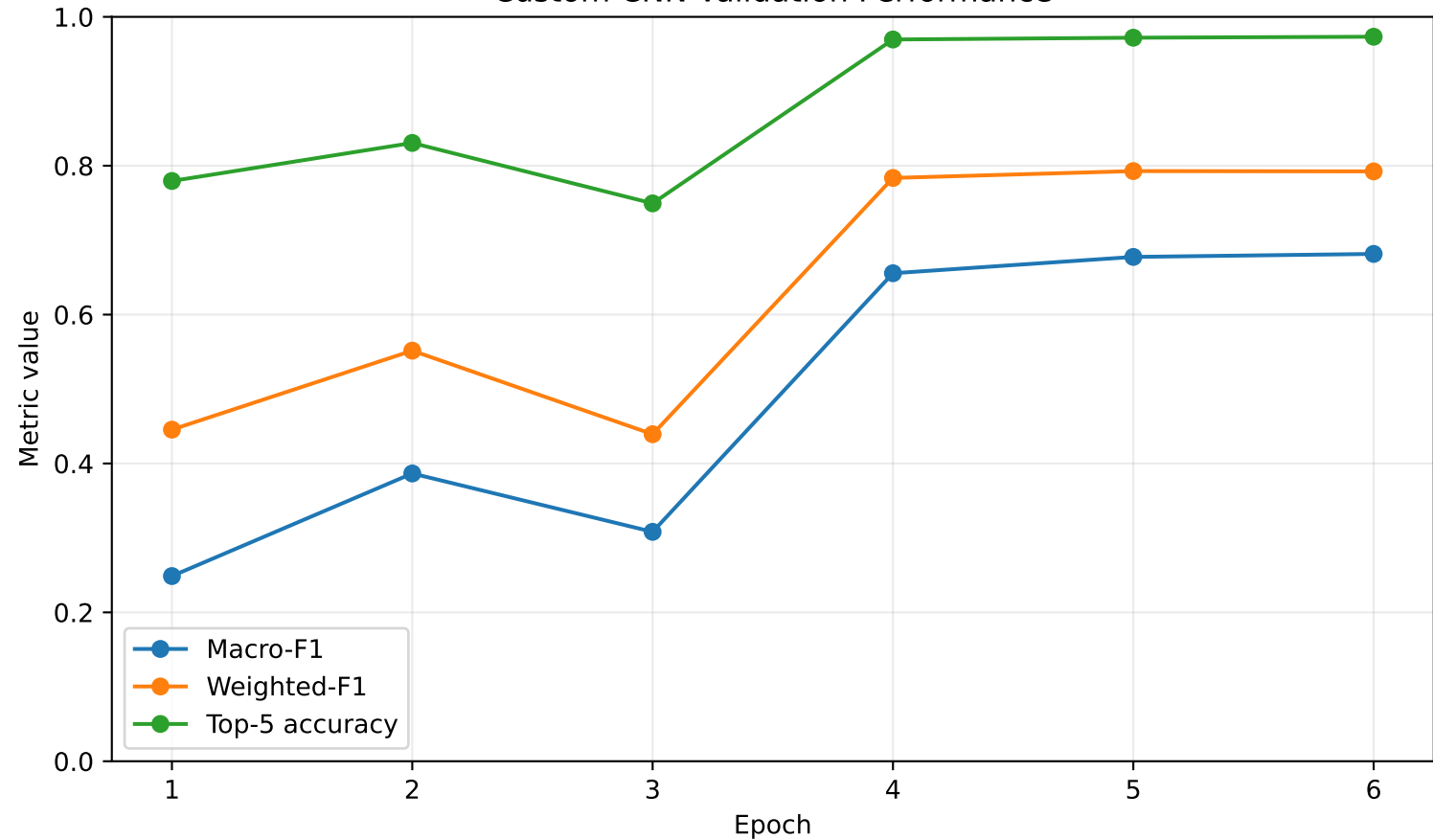
Custom CNN Validation Performance
