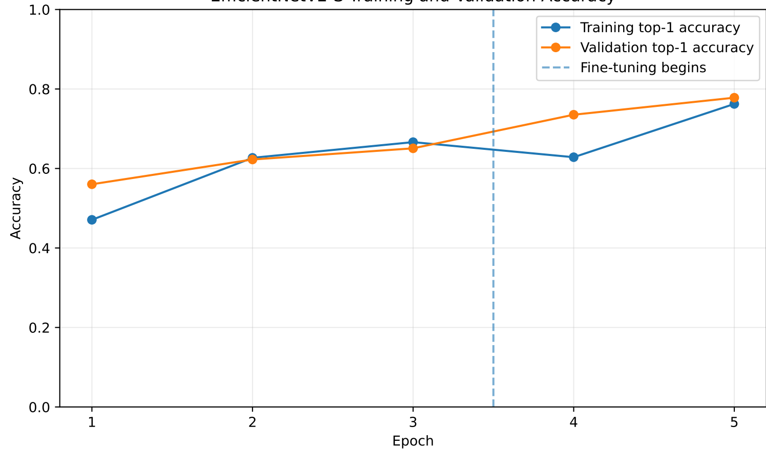
EfficientNetV2-S Training and Validation Accuracy
