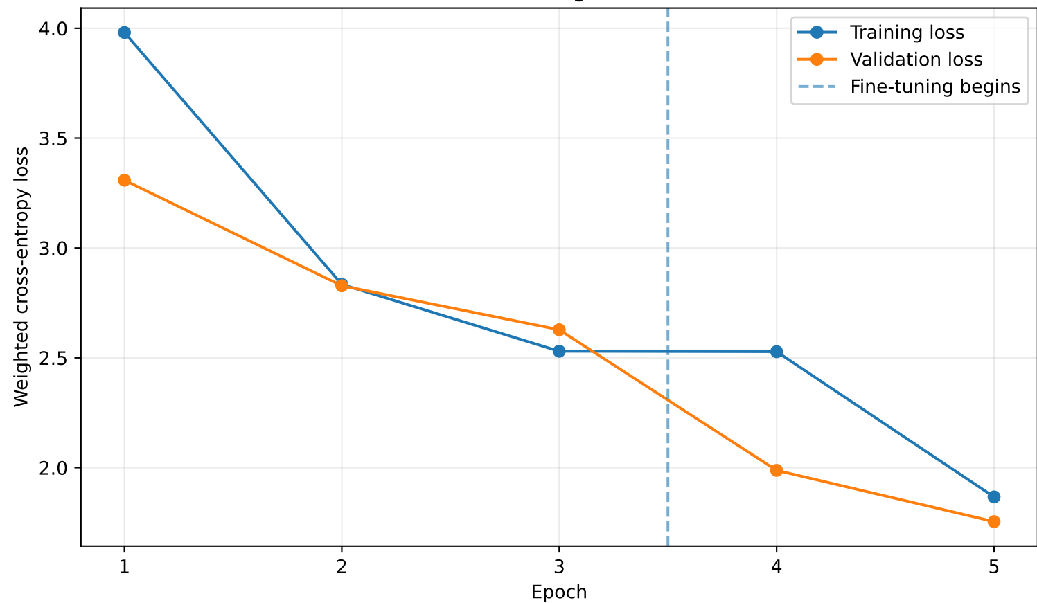
EfficientNetV2-S Training and Validation Loss
