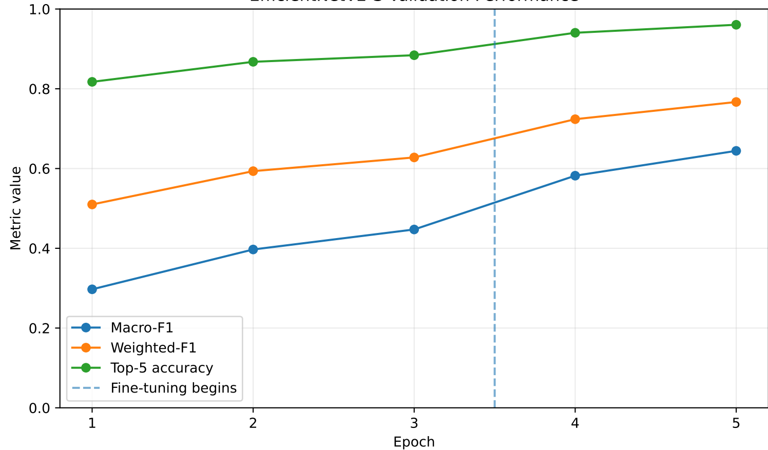
EfficientNetV2-S Validation Performance
