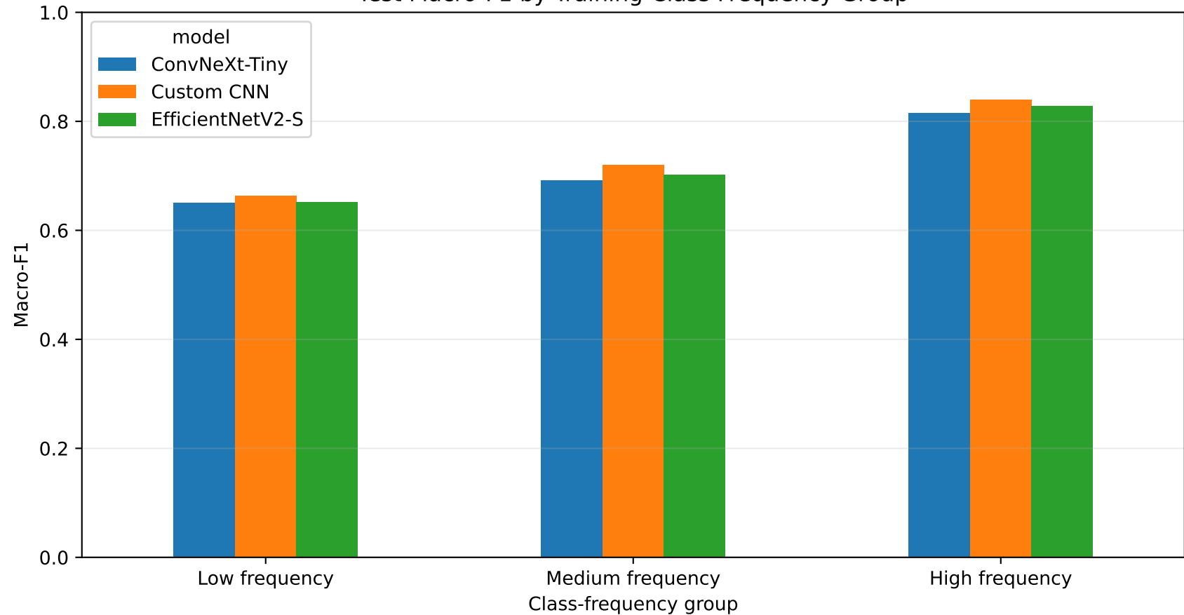
Test Macro-F1 by Training-Class Frequency Group
