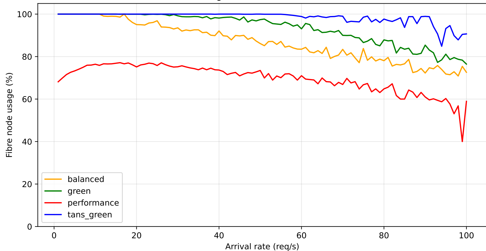
Fibre node usage - mobilenetv2 homo (3 nodes)
