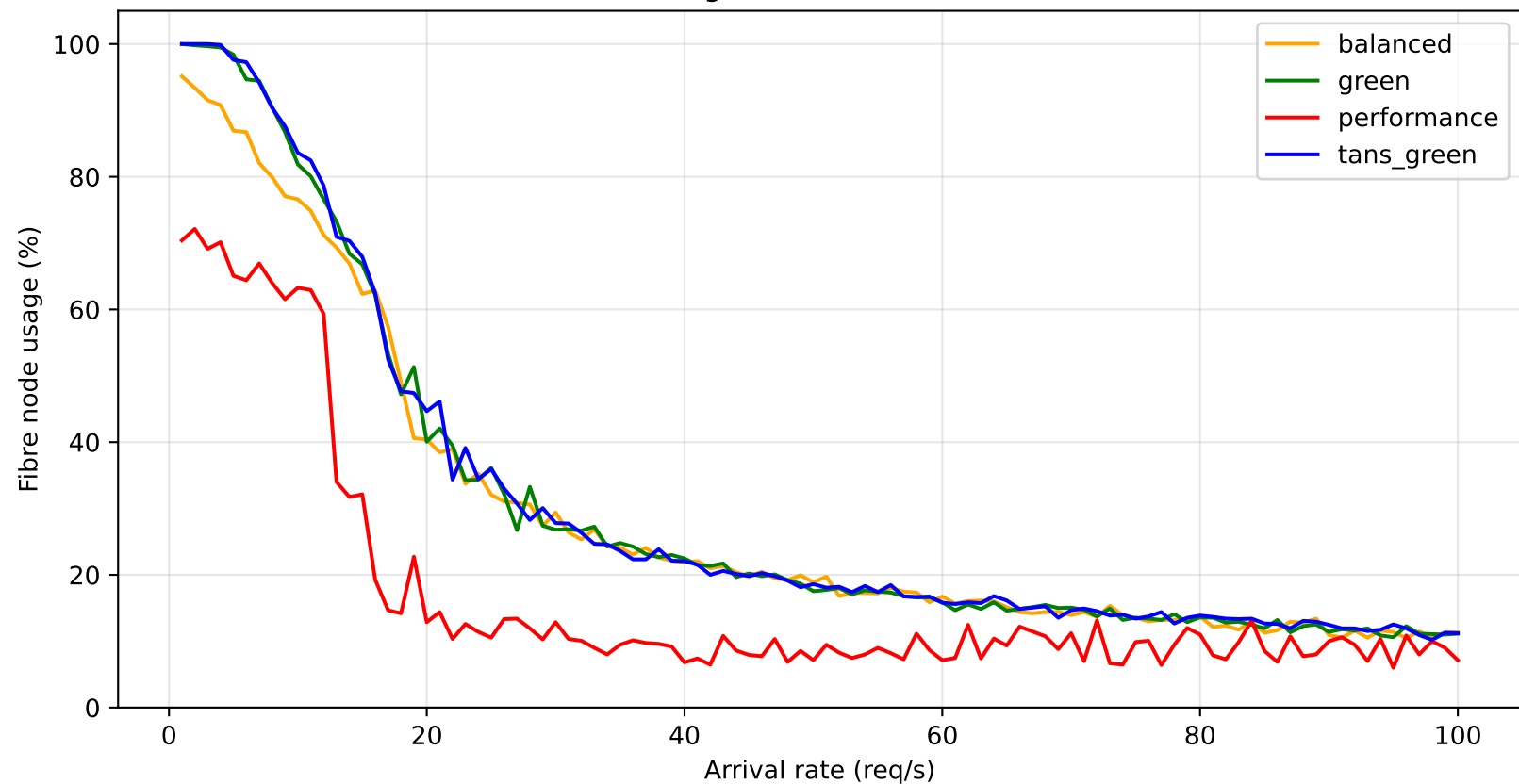
Fibre node usage - resnet50 homo (3 nodes)
