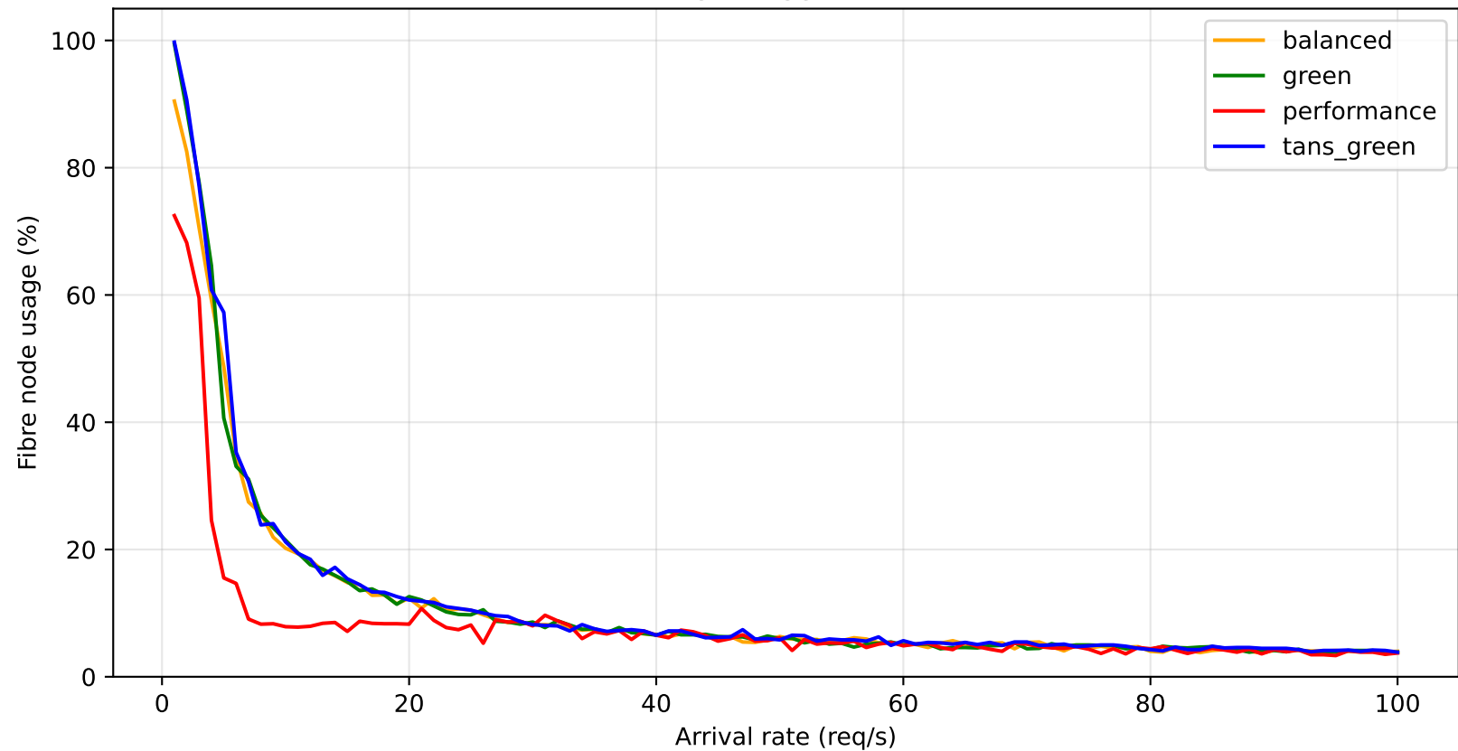
Fibre node usage - vgg16 homo (3 nodes)
