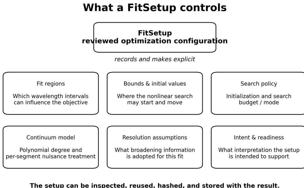
Figure 10.1. Main components controlled or recorded by a FitSetup. The purpose of the object is to make the optimization problem inspectable and reproducible rather than allowing fitting regions, bounds, search policy, continuum choices, resolution assumptions, and scientific intent to remain hidden defaults.
