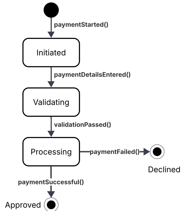
Payment Process State Diagram
