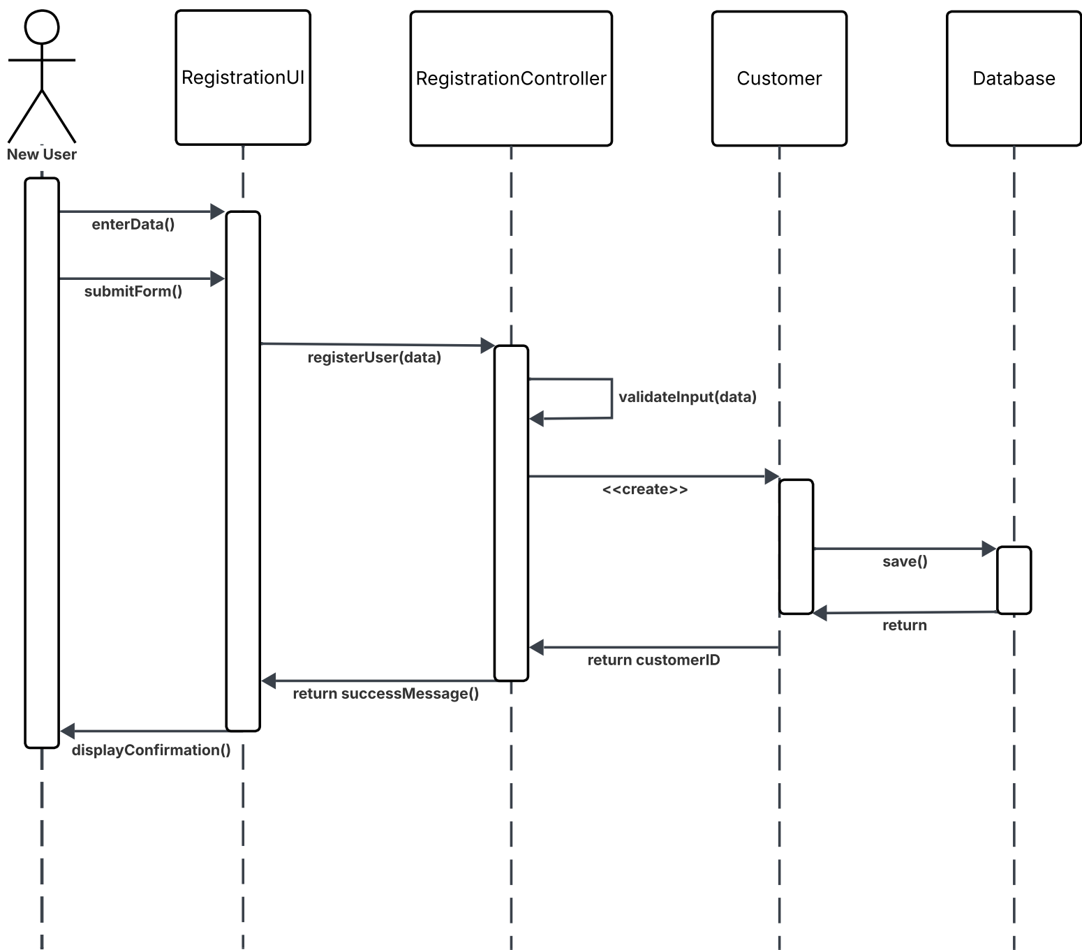
Registration Sequence Diagram
