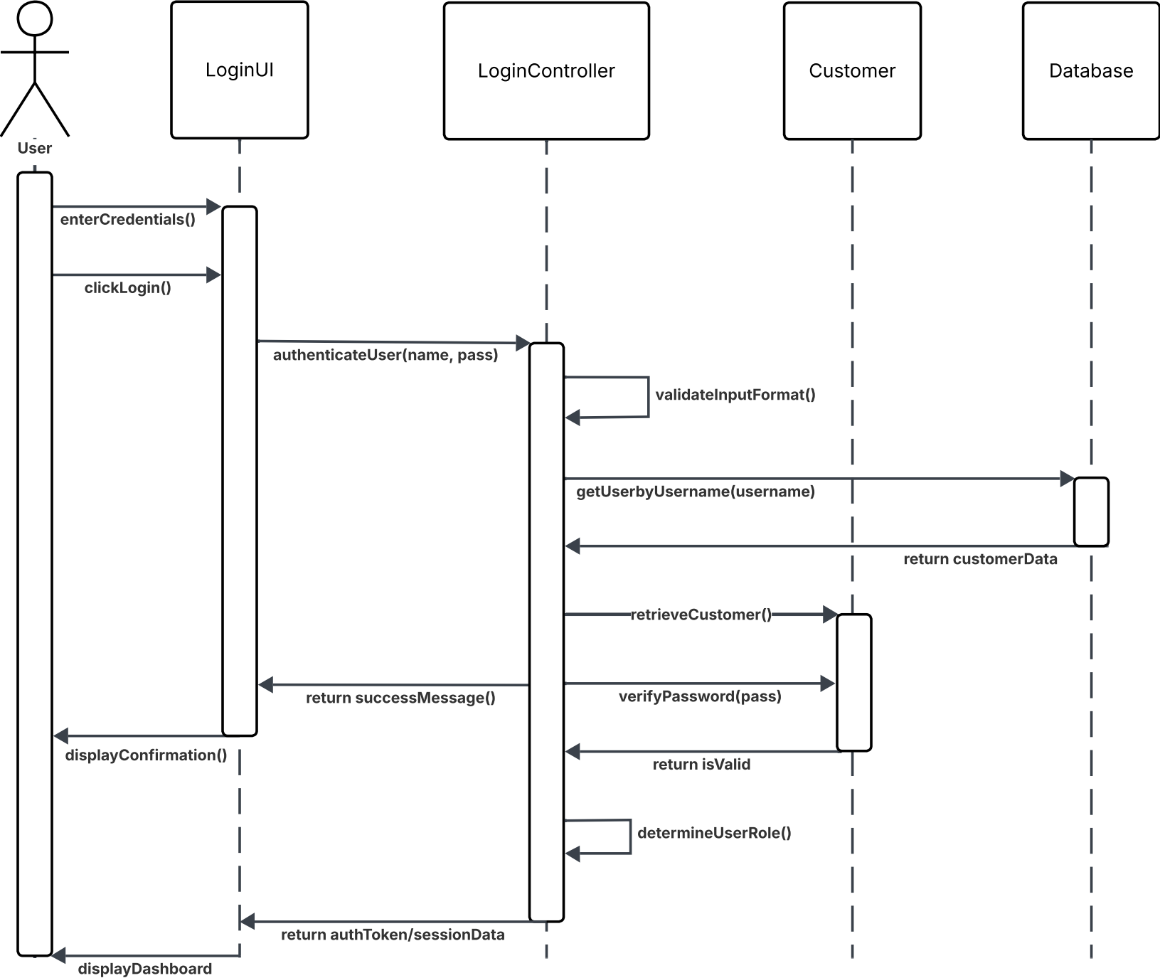
Login Sequence Diagram
