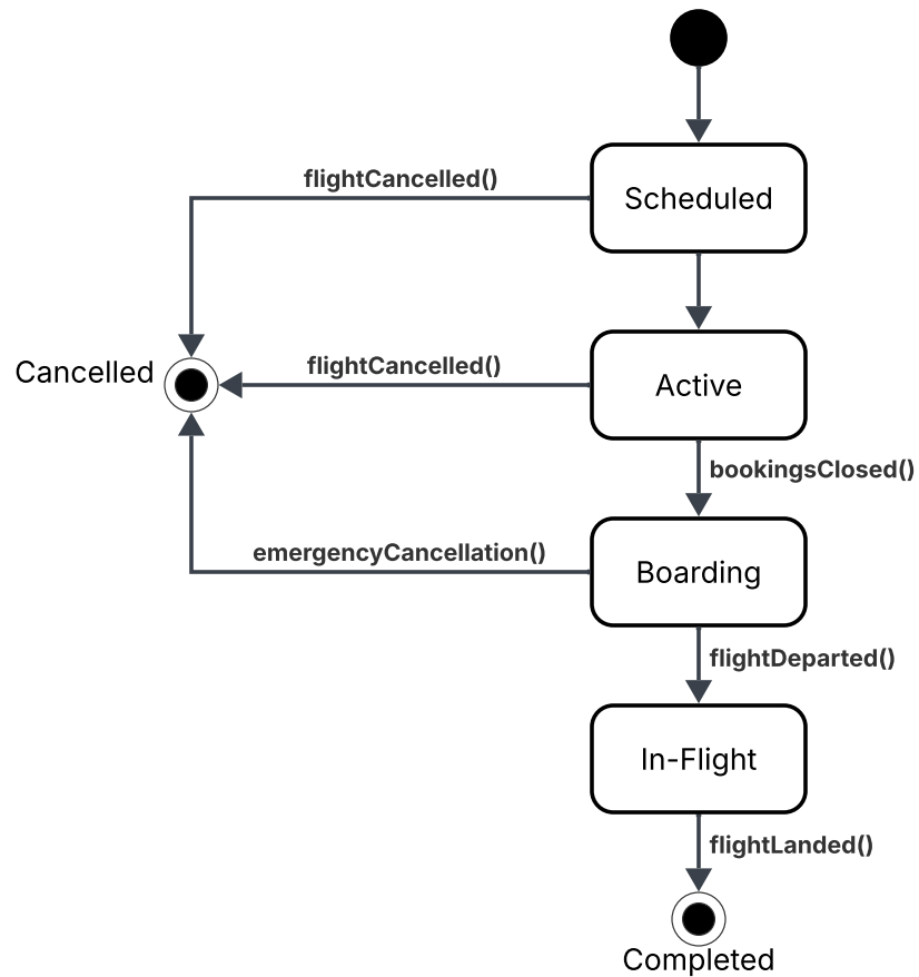
Flight Object State Transition Diagram
