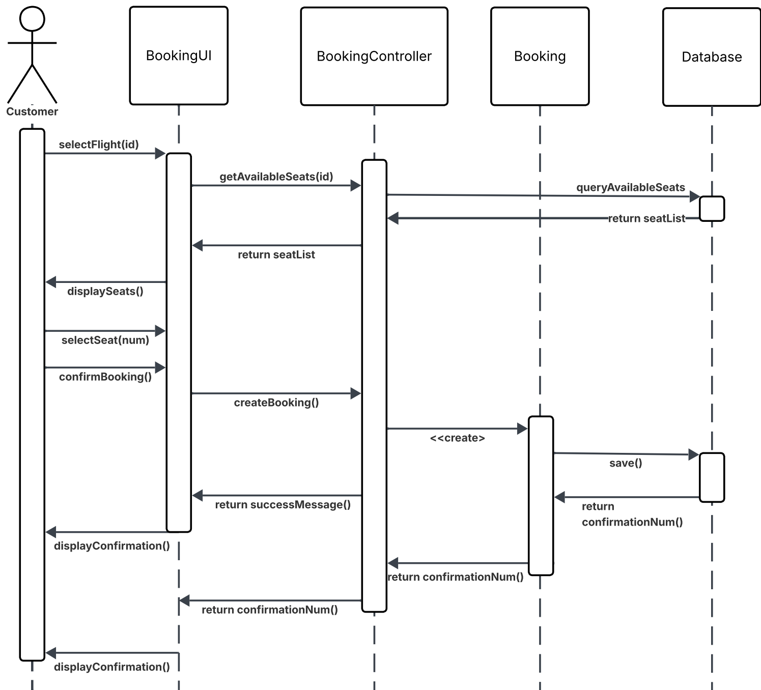
Flight Booking Sequence Diagram
