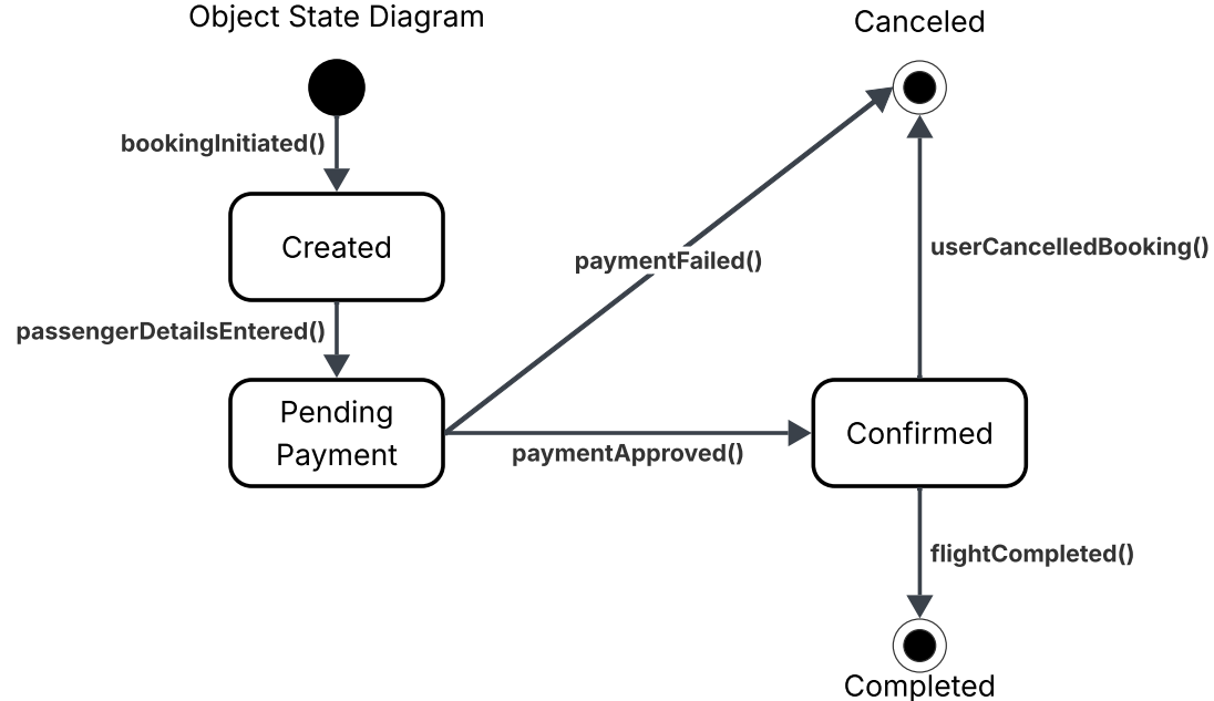
Booking/Reservation Object State Diagram
