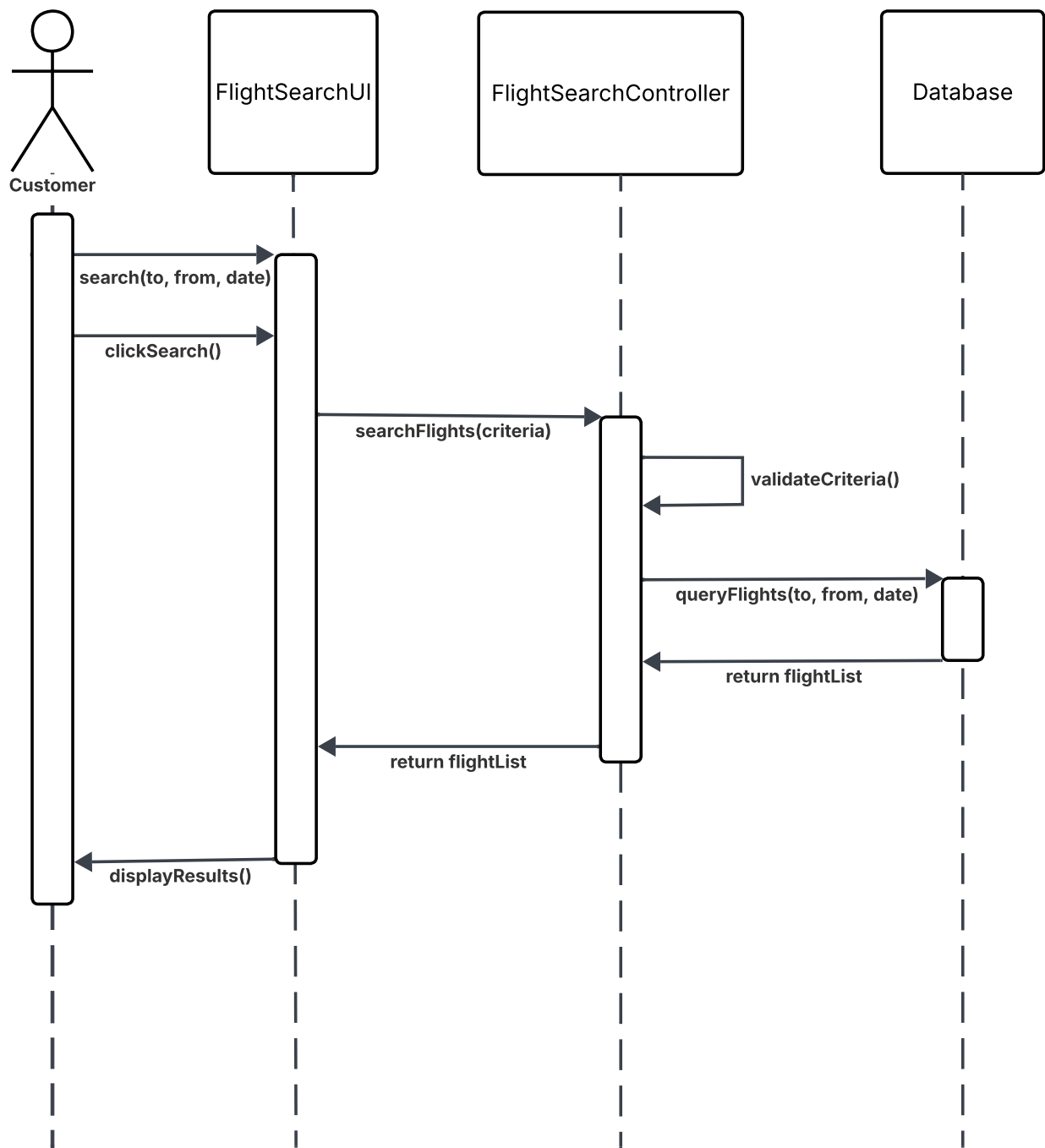
Search/Browse Flights Sequence Diagram
