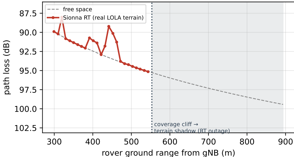
Connecting Ridge access channel — Sionna RT on PGDA LOLA 5 m/px
