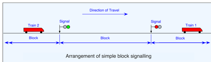
Figure 2.5: Simplified block signalling principle
