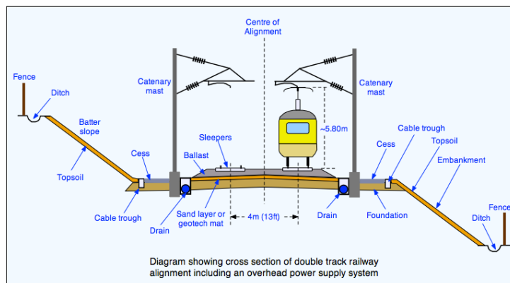
Figure 3.2: Schematic representation of railway infrastructure components.
