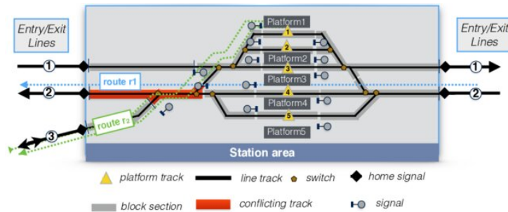
Figure 3.5: Example of a station layout
