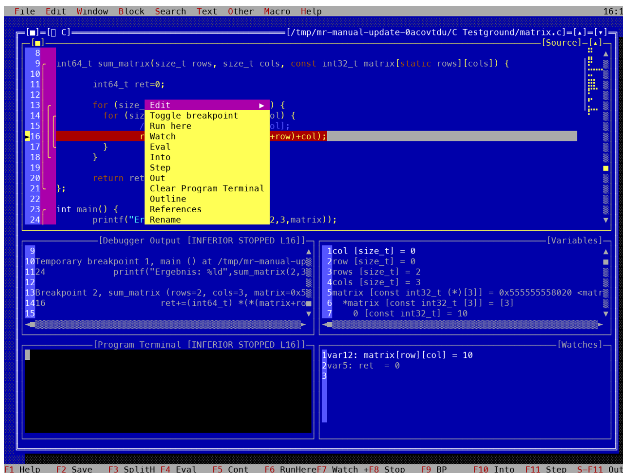
Figure 23.2: PTY capture of the extended GDB source menu in a paused matrix.c session. Watch uses the clicked identifier; Into, Step, and Out act on the current execution stop.
