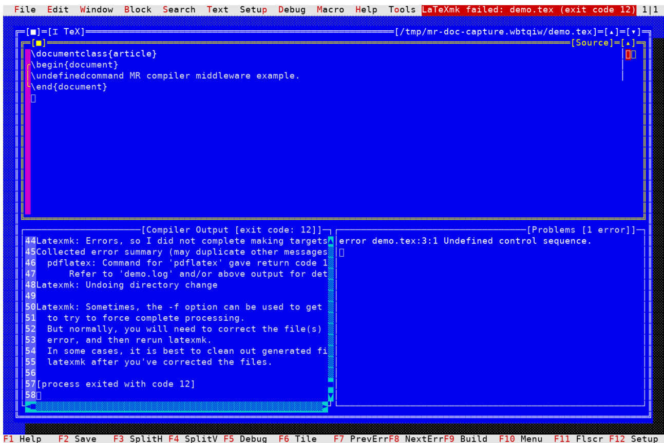
Figure 23.3: An intentionally invalid TeX source after the LaTeXmk build. The Problems pane shows the compiler diagnostic; the red message reports the post-build macro's failure branch. No PDF viewer is started on this branch.
