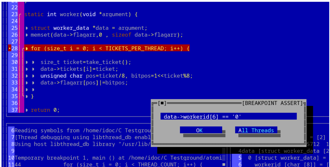
Figure 23.5: The Breakpoint Assert dialog for a source breakpoint. All Threads removes the condition; closing the dialog leaves it unchanged.
