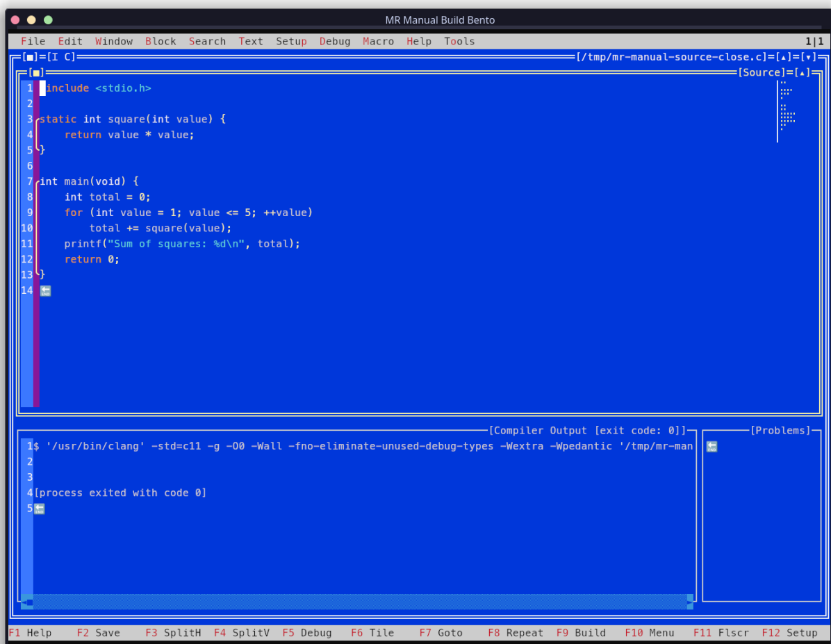
Figure 23.4: The build Bento with the Source pane’s inner close button. It returns to the source editor; the separate button on the outer window frame closes the window after the usual unsaved-change check.
