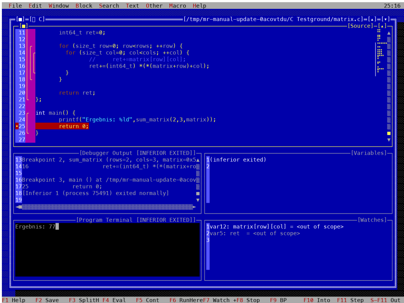
Figure 23.9: PTY capture after matrix.c finishes. Program Terminal retains Ergebnis: 77 ; debugger status and program output occupy separate panes.
