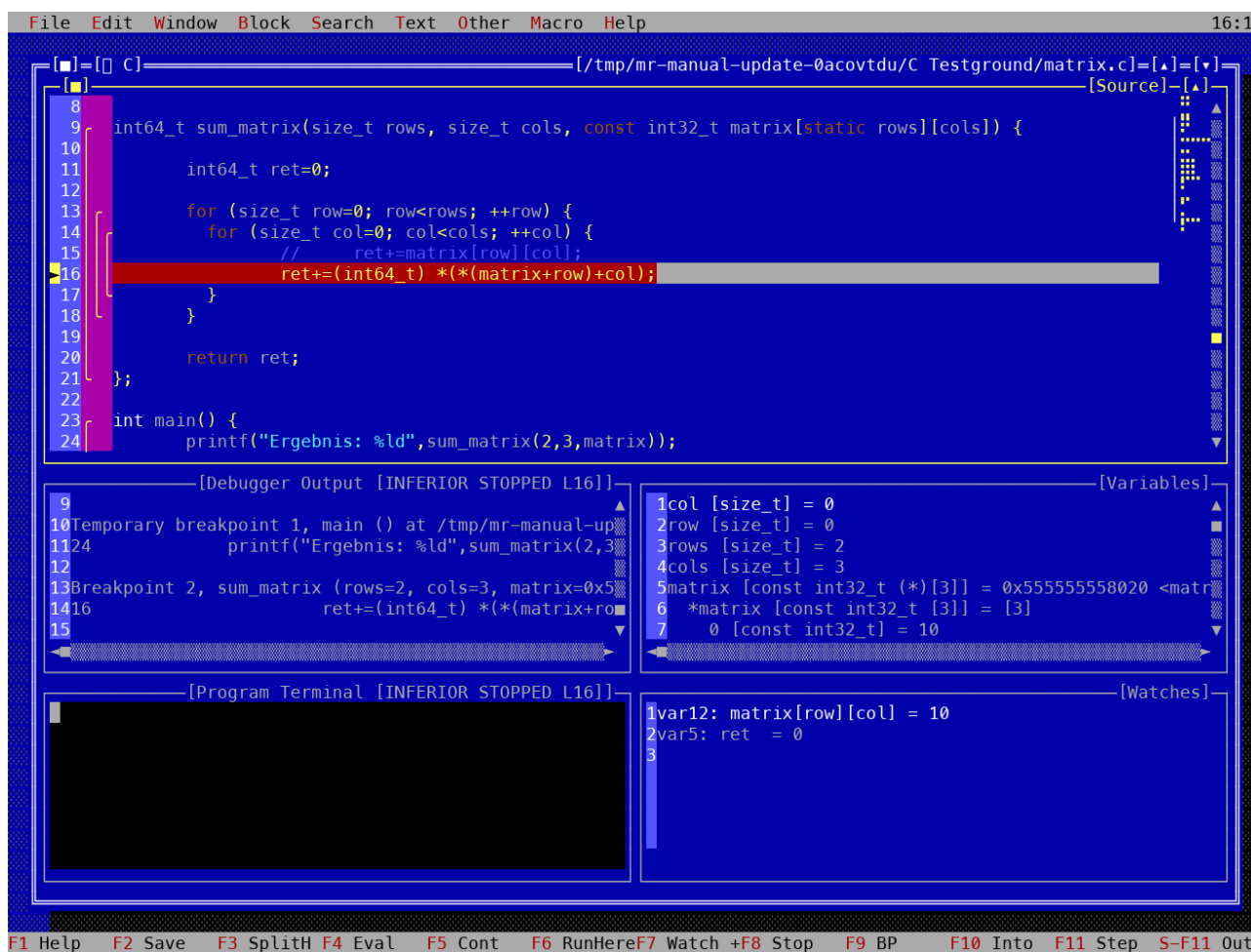
Figure 23.8: PTY capture of matrix.c paused inside sum_matrix . The source position, Variables, and Watches describe the same stop; Program Terminal is a separate pane.
