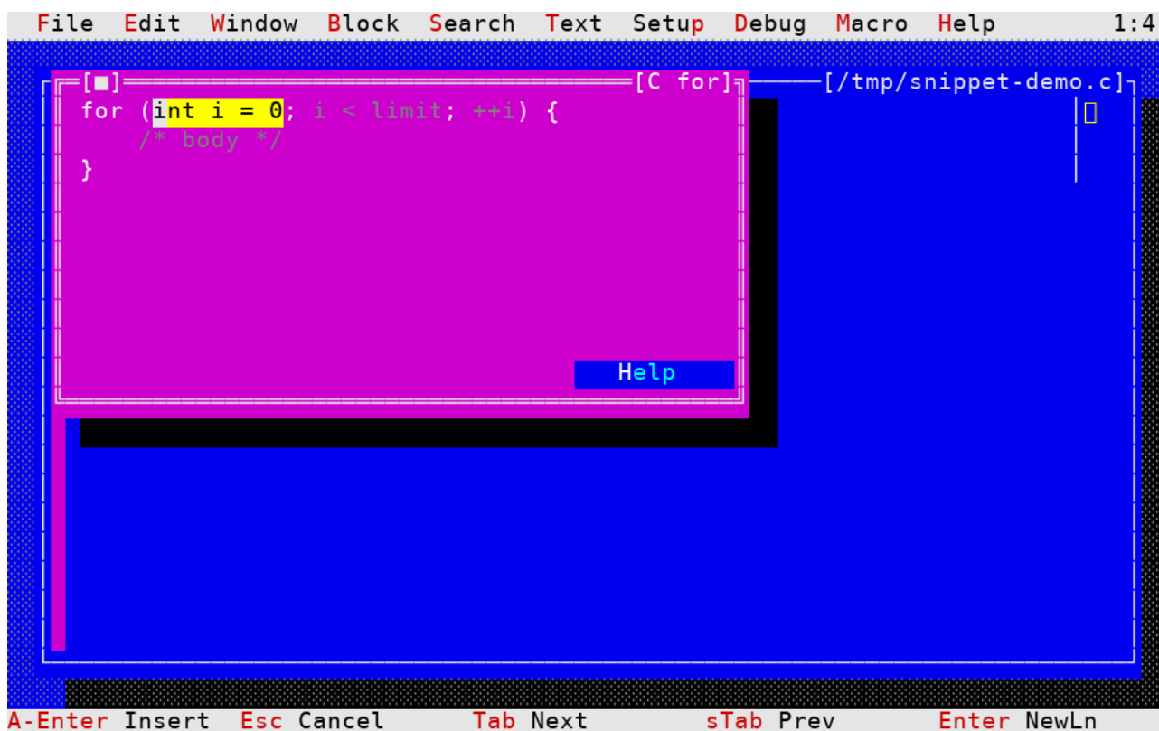
Figure 7.1: The C for expansion opens in the Snippet SideKick. The first placeholder is highlighted; the command line lists Insert, Cancel, Next, and Previous.
