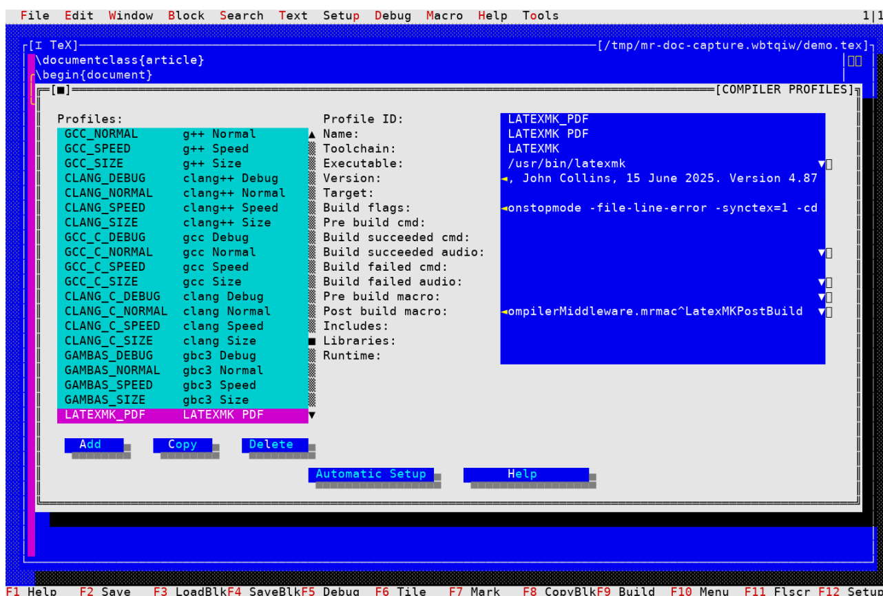
Figure 23.2: The Compiler Profiles dialog with the LaTeXmk profile selected. Its Post build macro field names the bundled routine that handles the completed PDF build.
