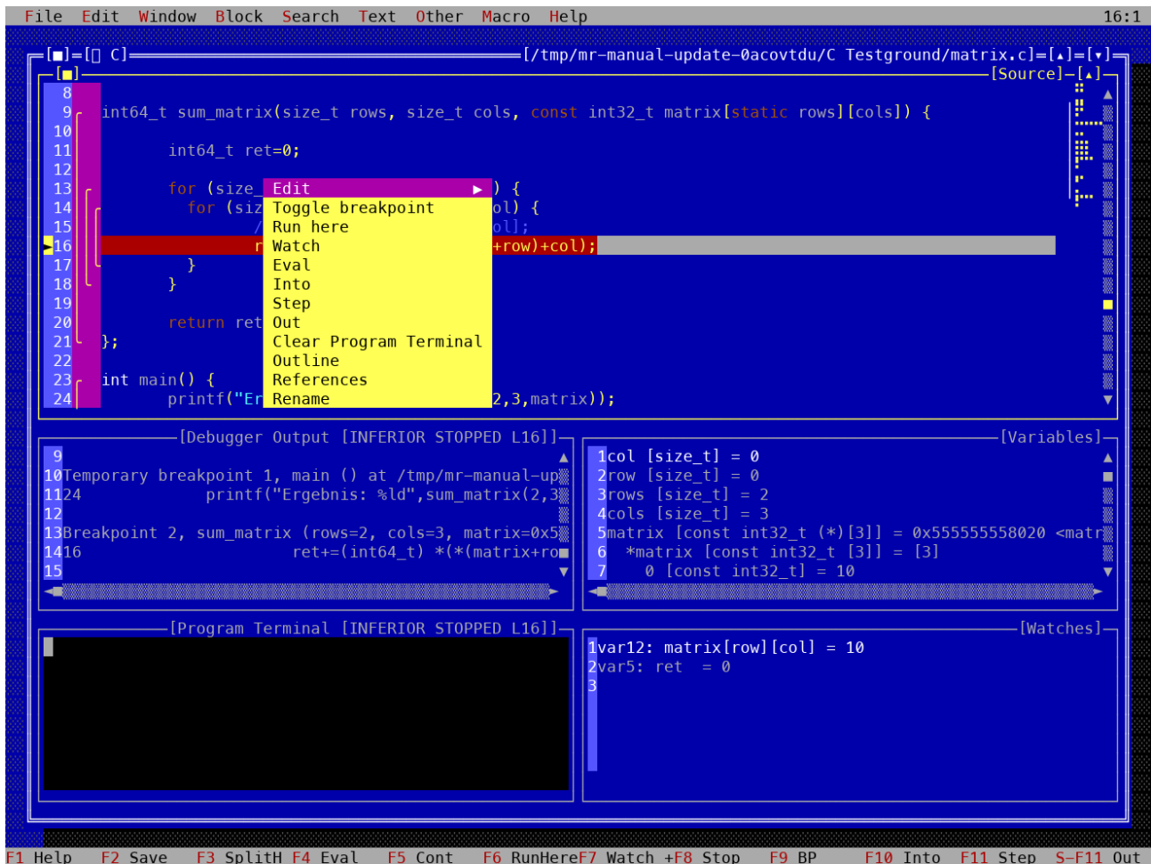
Figure 23.7: PTY capture of the extended GDB source menu on a line without a breakpoint in a paused matrix.c session. Watch uses the clicked identifier; Into, Step, and Out act on the current execution stop.
