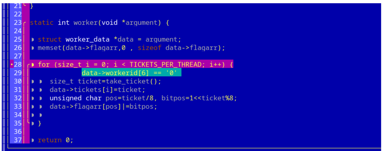
Figure 23.6: The Source pane shows the assertion of the breakpoint under the pointer using the same transient hint style as the frame markers.
