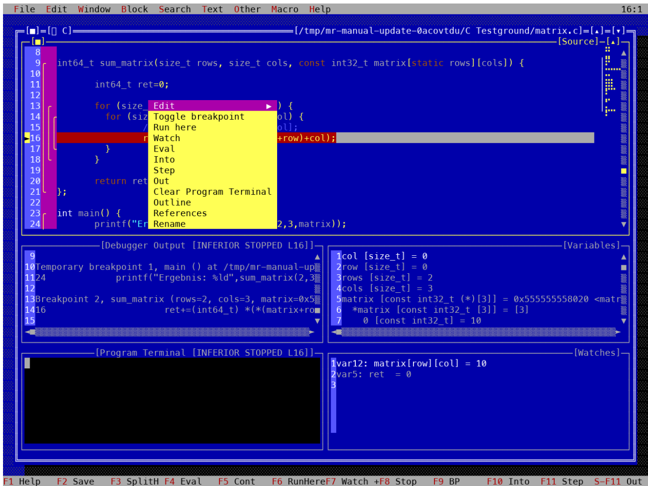
Figure 23.2: PTY capture of the extended GDB source menu in a paused matrix.c session. Watch uses the clicked identifier; Into, Step, and Out act on the current execution stop.
