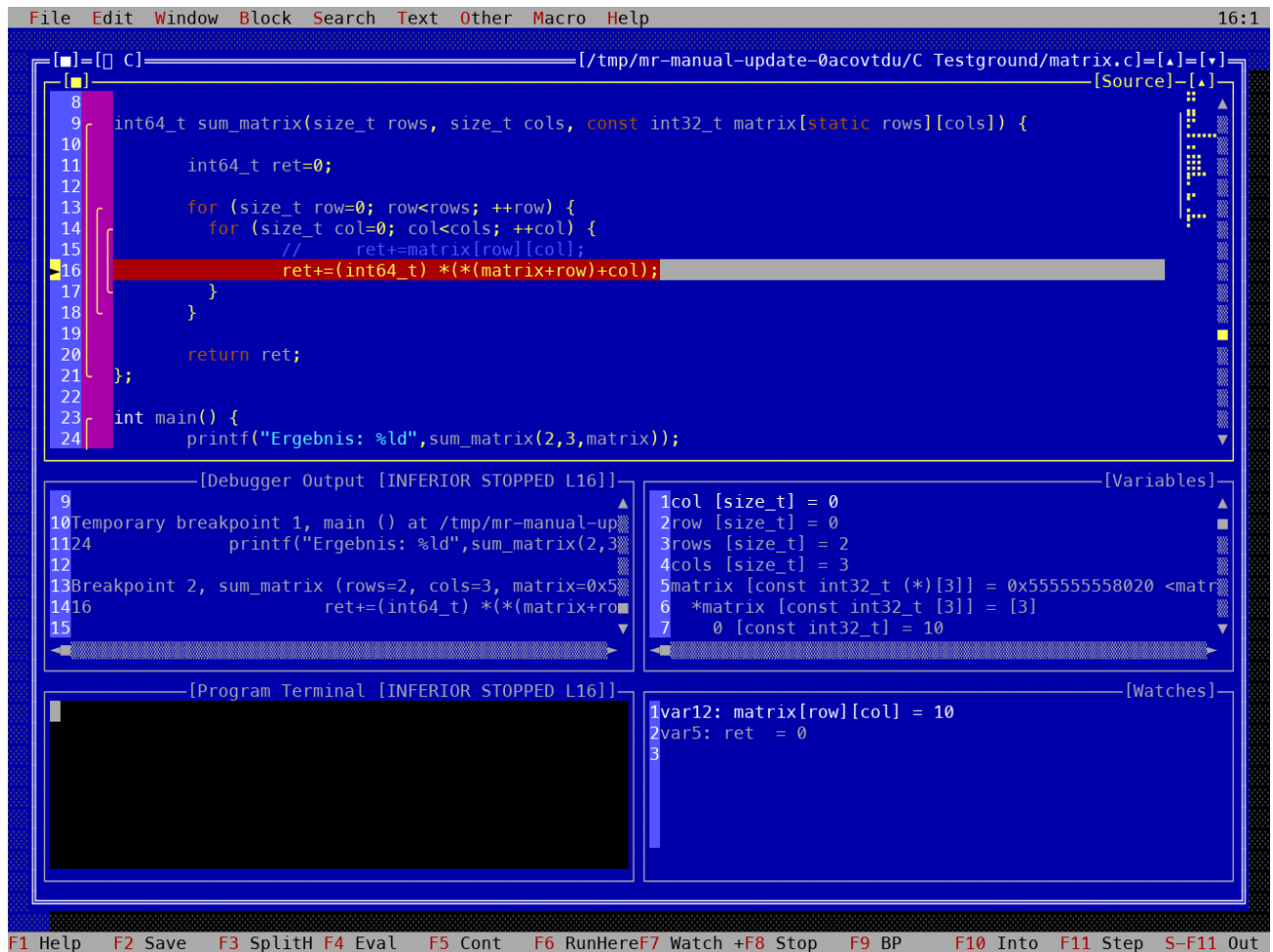
Figure 23.3: PTY capture of matrix.c paused inside sum_matrix . The source position, Variables, and Watches describe the same stop; Program Terminal is a separate pane.
