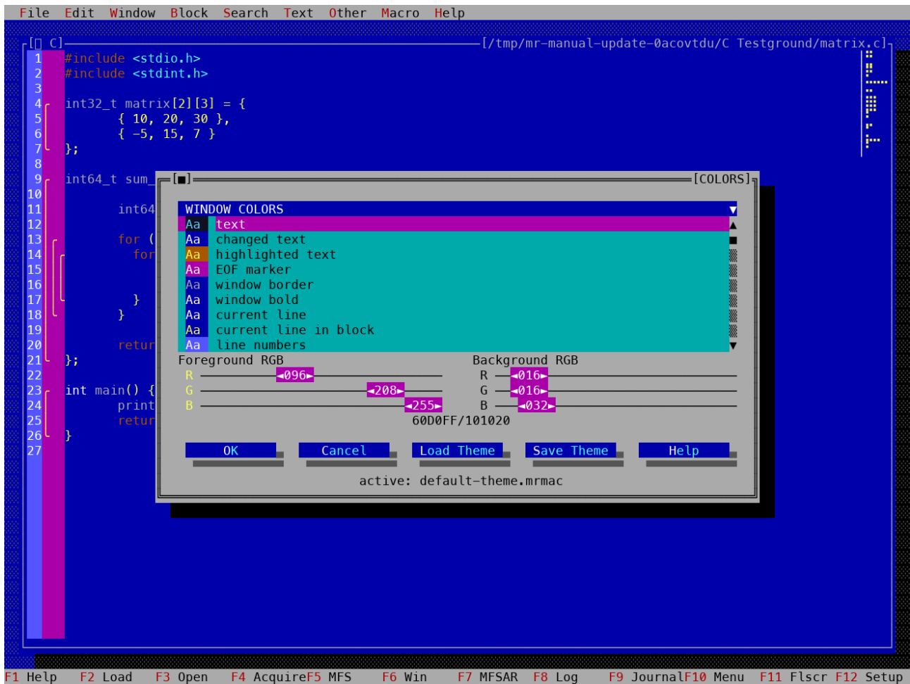
Figure 4.2: PTY capture of Color setup with 24-bit RGB output selected. Foreground and background have separate RGB sliders. The displayed 60D0FF/101020 pair and the text-role sample update immediately, including while a slider is being dragged.
