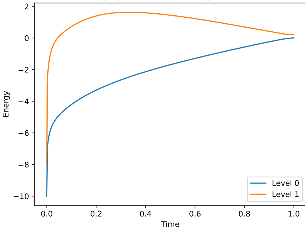
Energy spectrum for n=10 , \gamma=1.0
