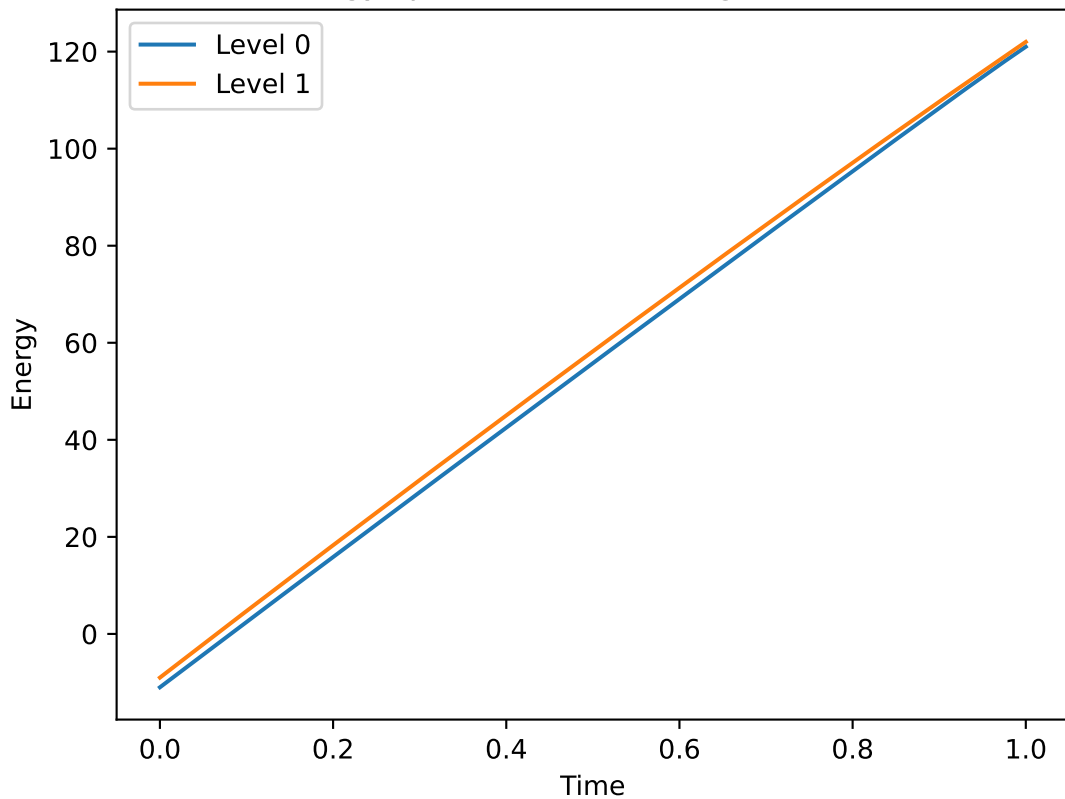
Energy spectrum for n=11 , \gamma=1.0
