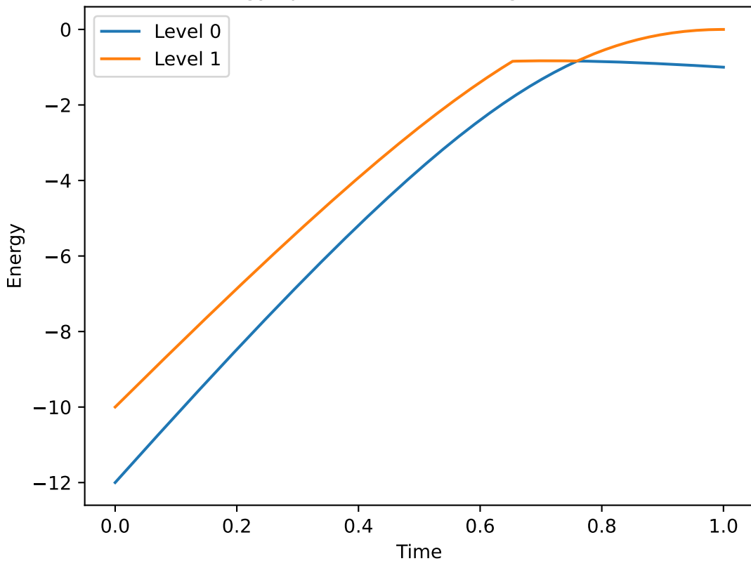
Energy spectrum for n=12 , \gamma=1.0
