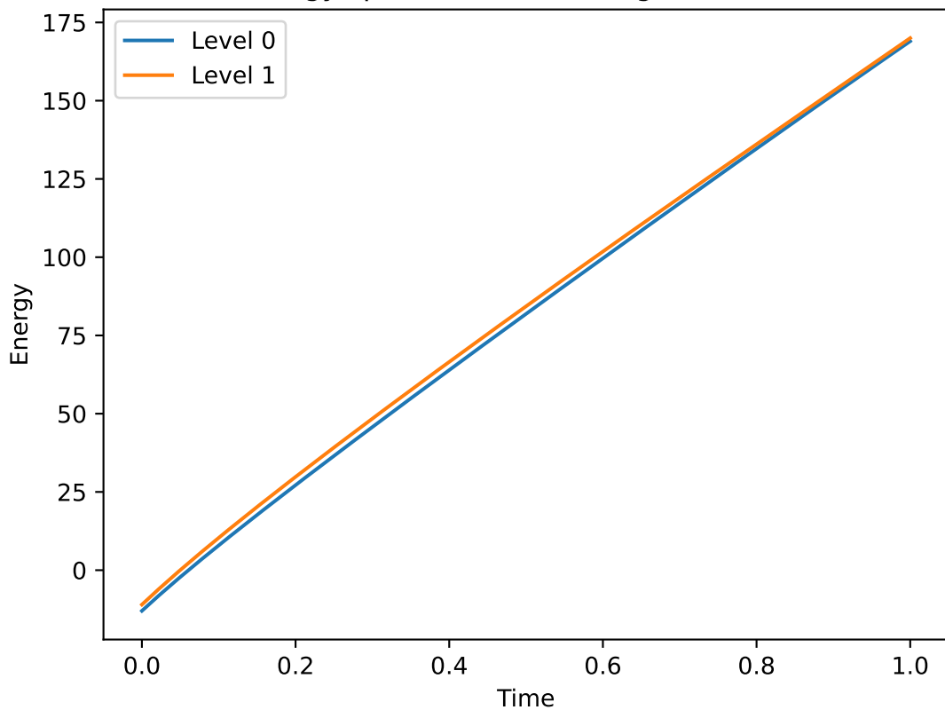
Energy spectrum for n=13 , \gamma=1.0
